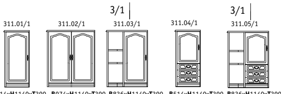
В514xH1140xT390 В974xH1140xT390 В836xH1140xT390 В514xH1140xT390 В836xH1140xT390
