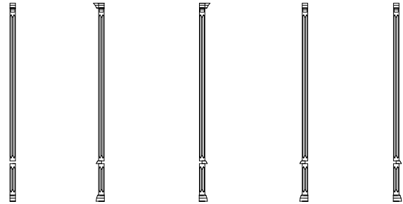
B68(0)xH2450xT388 B132(98)H2450xT388 B98H2450xT388 B132(98)H2450xT388
